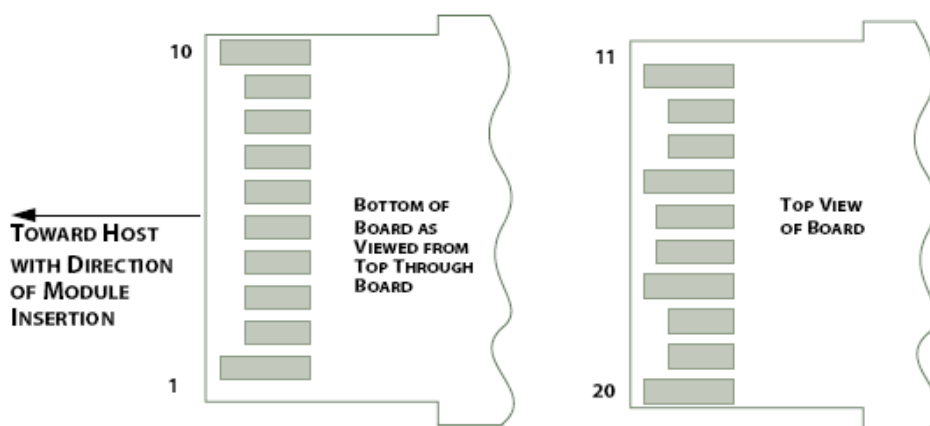
Figure 3: Module Contact Assignments
