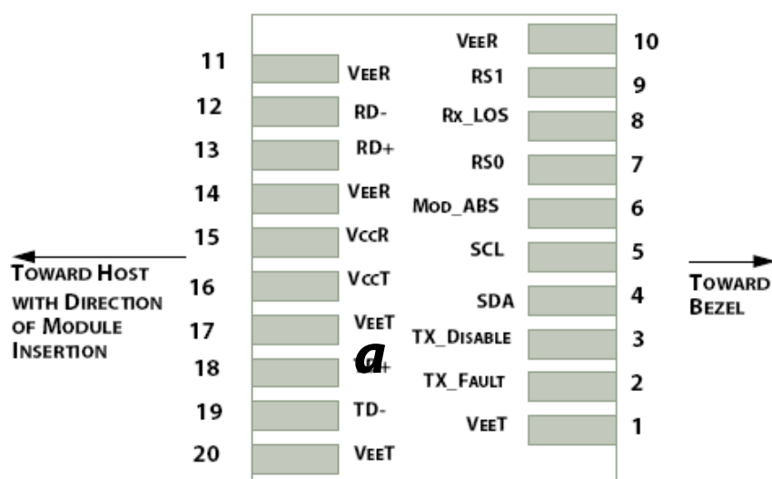
Figure 2: Host PCB Contacts
